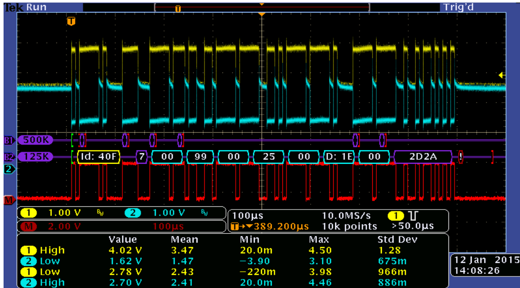
DupMac @ 125K, 11VDC
