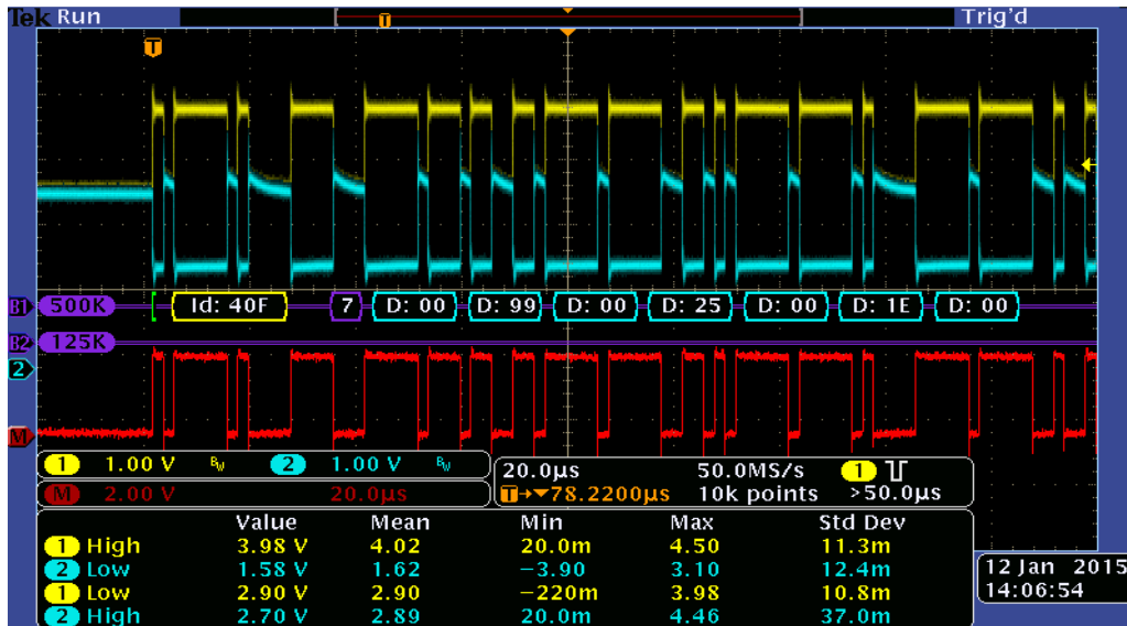
DupMac @ 500K, 25VDC
